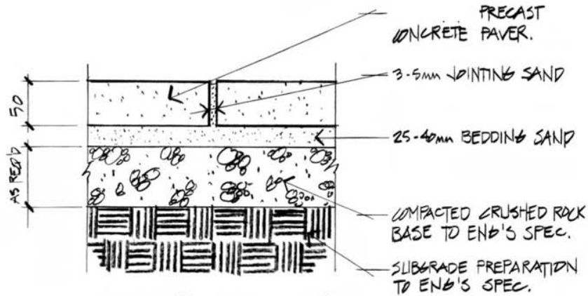
SECTION - PEDESTRIAN FLEXIBLE PAVING SYSTEM 1:5
