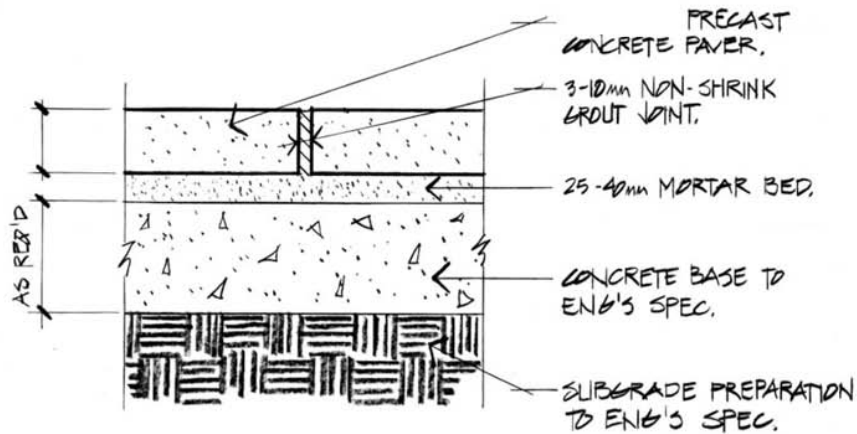
SECTION - PEDESTRIAN RIGID PAVING SYSTEM 1:5
